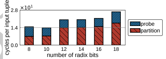
Figure 18: Impact of number of radix bits ( \#r ) of PRJ.
