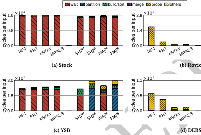
Figure 7: Execution time breakdown.
