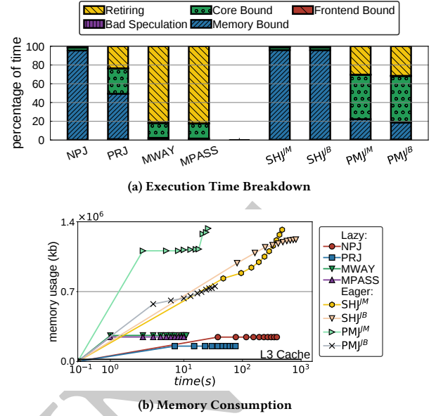
Figure 19: Micro-architectural Analysis on Rovio.
