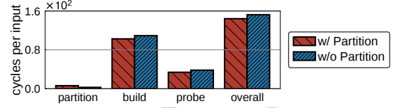
Figure 17: Impact of physical partitioning of SHJ JM .
