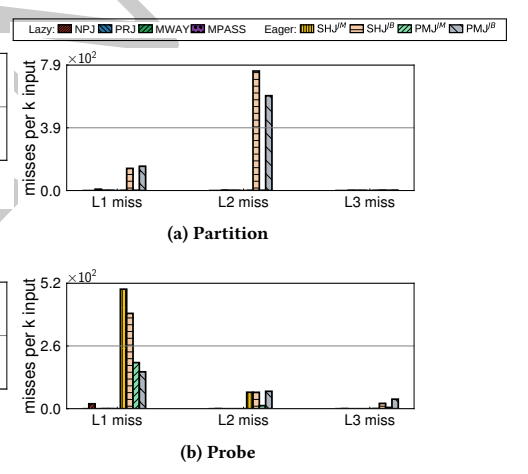
Figure 8: Cache efficiency profiling (YSB).
