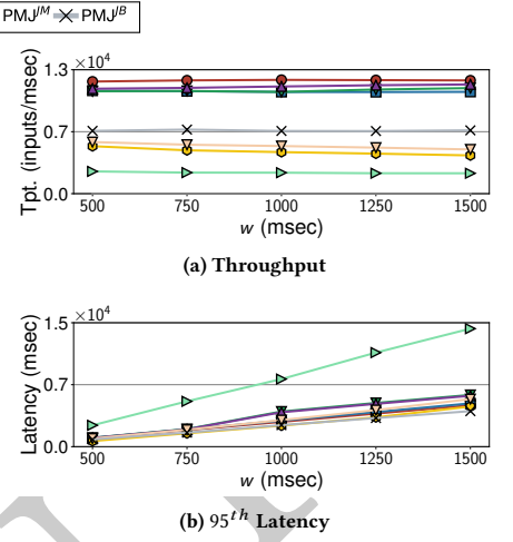
Figure 14: Impacts of window length ( v = 12800 ).
