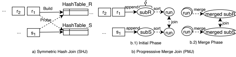
Figure 1: Stream join algorithms.
