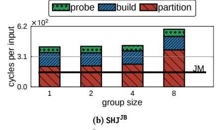
Figure 16: Impact of group size ( g ).
