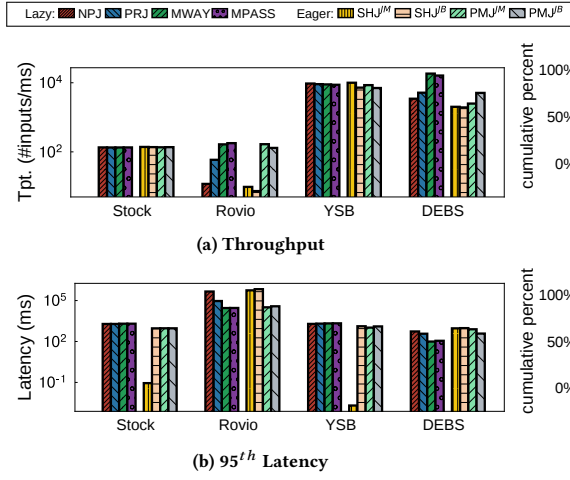
Figure 5: Throughput and latency comparison.
