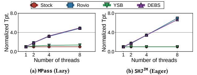
Figure 20: Impact of multicores.
