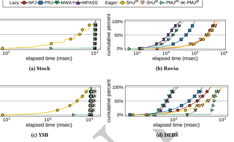
Figure 6: Progressiveness comparison.
