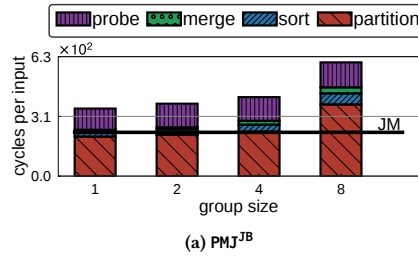
Figure 16: Impact of group size ( g ).
